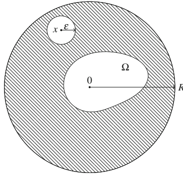
Fig. 43.1 Geometric illustration of x \notin \Omega , B_\varepsilon(x) and B_R(0) .
